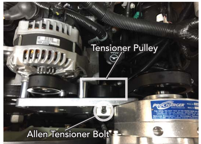
Belt Tensioner
