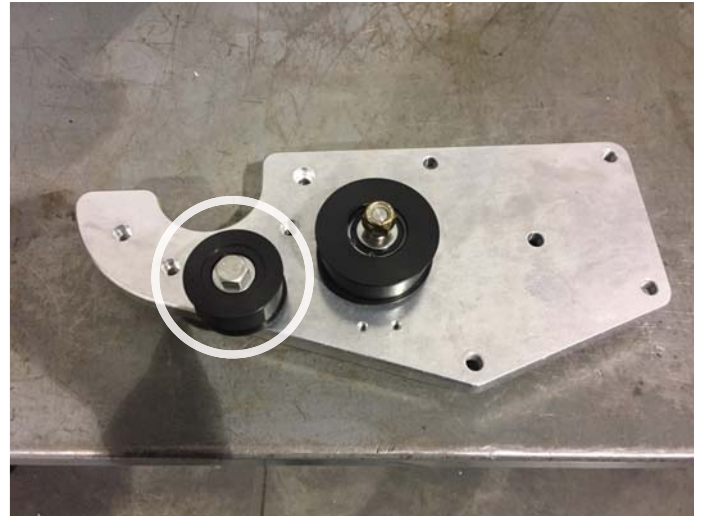
Remove Idler Pulley
