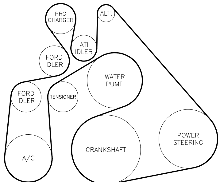
Belt-Routing Diagram
