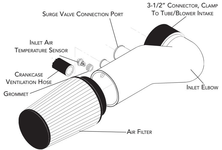
Supercharger Inlet Assembly
