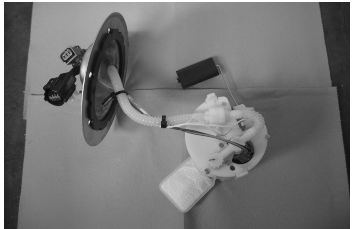
Fuel Pump Canister Assembly
