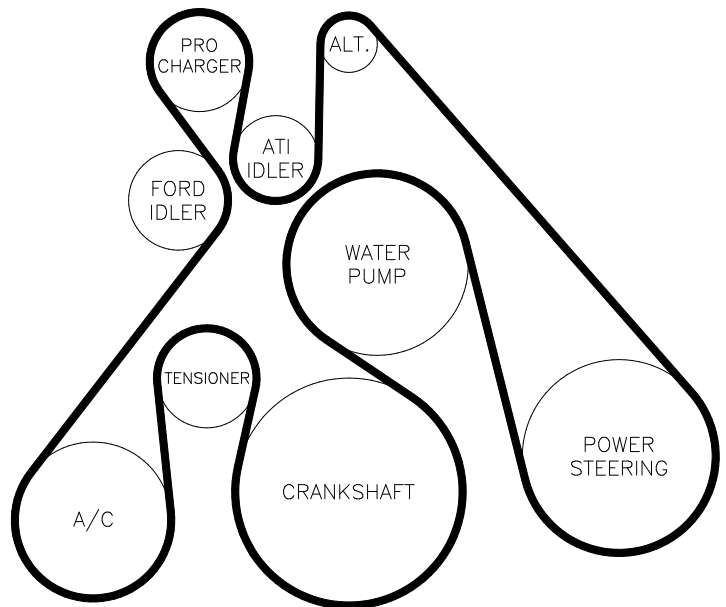
Belt-Routing Diagram
