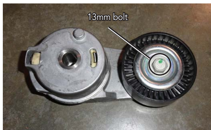
Tensioner Pulley Bolt
