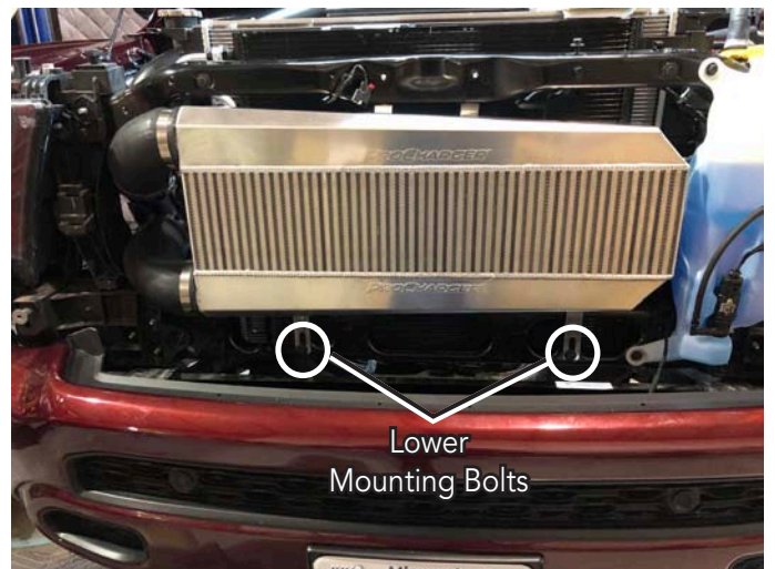
Intercooler Installed
