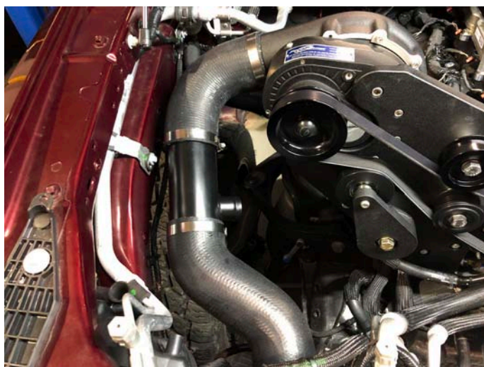
Tubing To Supercharger Installed
