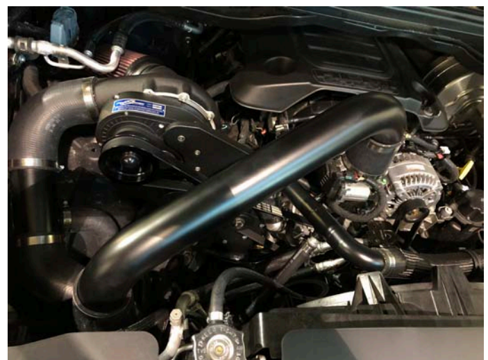
Throttle Body Tube Installed
