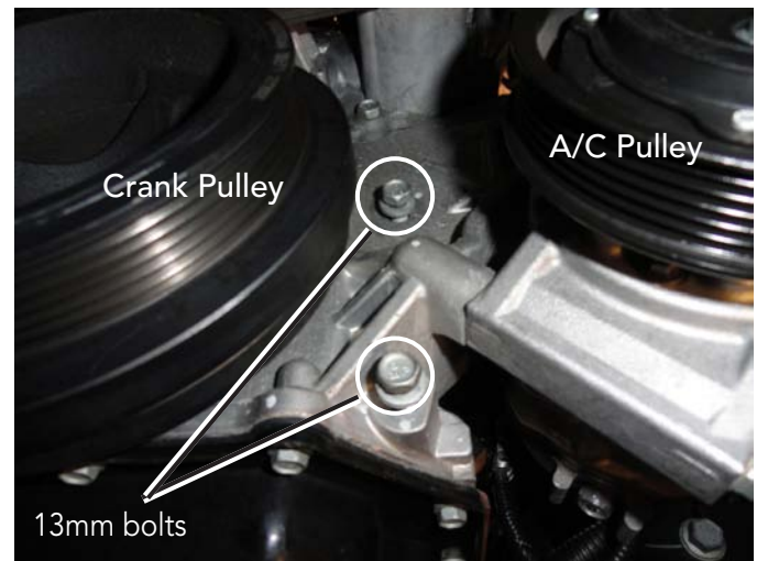
Front Cover Bolts
