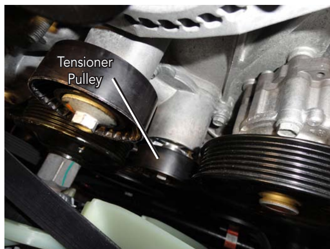
Installed Tensioner Pulley
