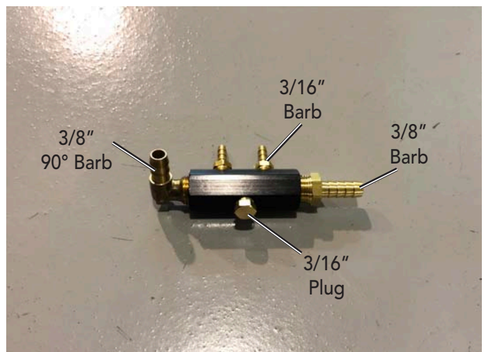
Vacuum Manifold
