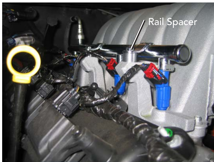
Fuel Rails Installed
