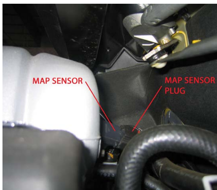
2 Bar MAP Sensor Installed (6.1L Model)
