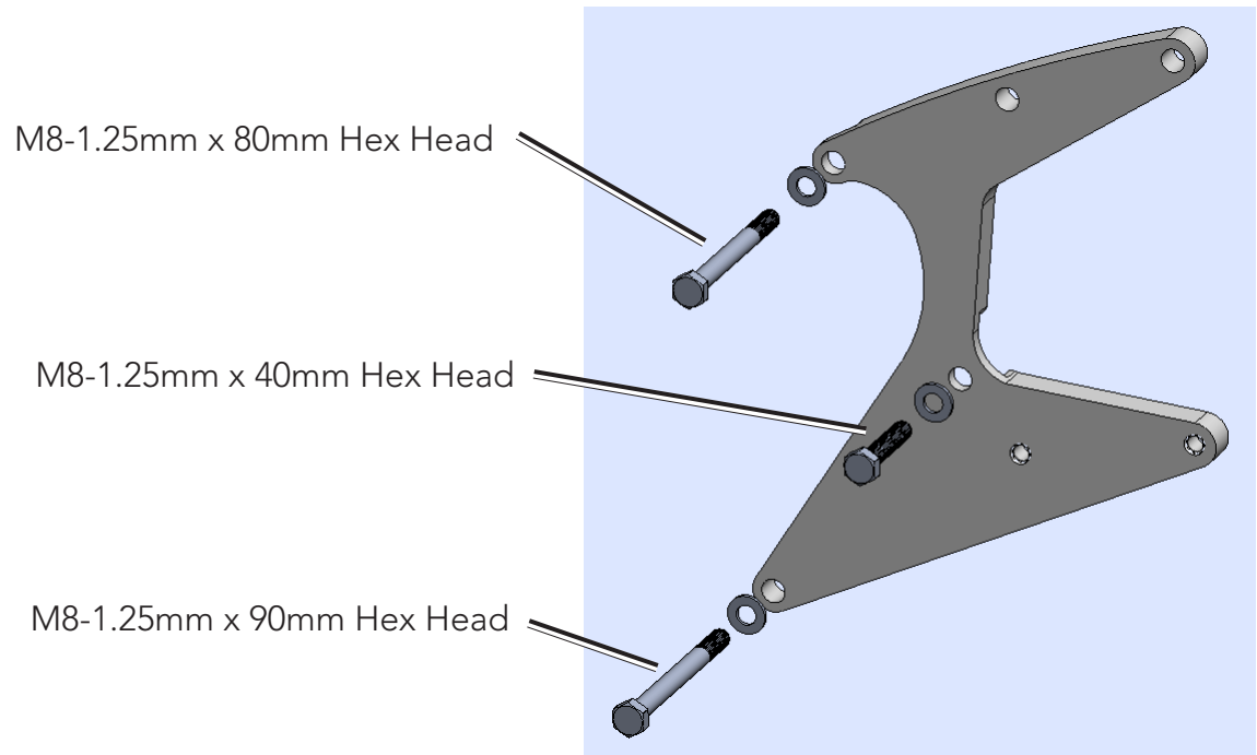
Sub-Bracket Installation
