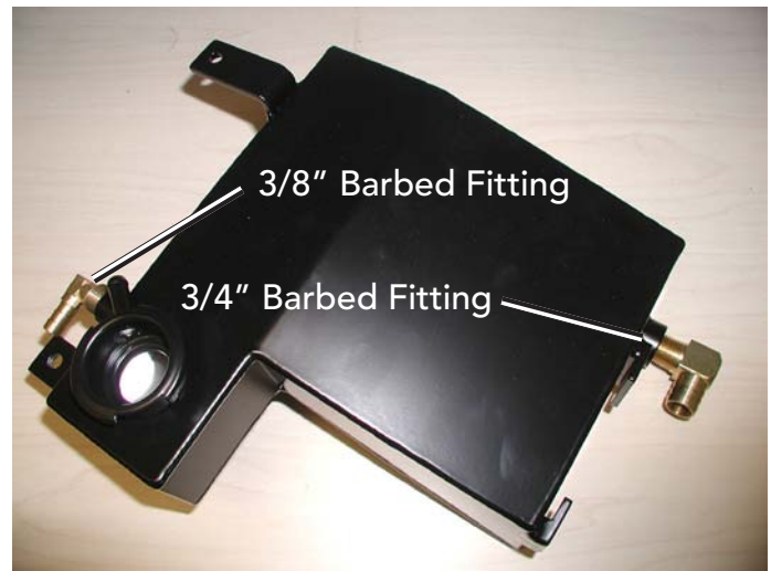
Supplied Coolant Reservoir
