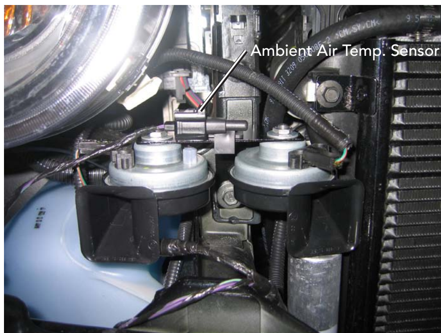
Horn Relocation
